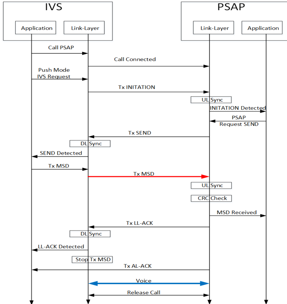
Figure 28: The EU emergency call BER test procedure.
