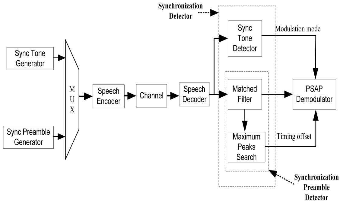
Figure 38: Block diagram of the synchronization frame generation, transmission, and detection for the up-link channel in the 3GPP eCall system.
